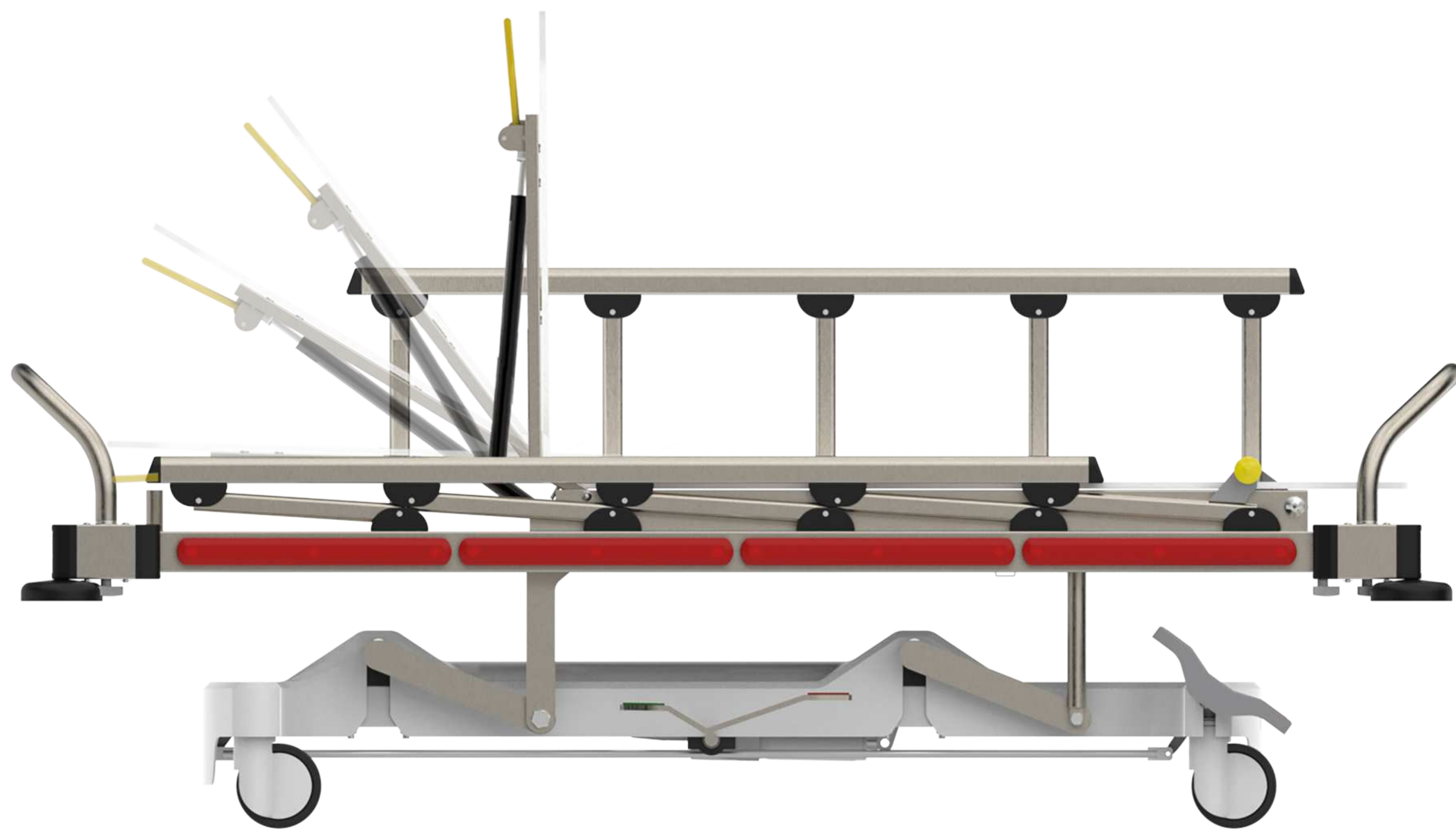
90° Backrest Movement
